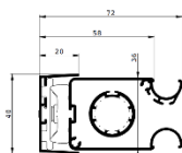
Mosquitera Enrollable FLEXA 1 hoja
